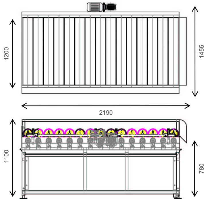
15 roller 1200mm wide model
